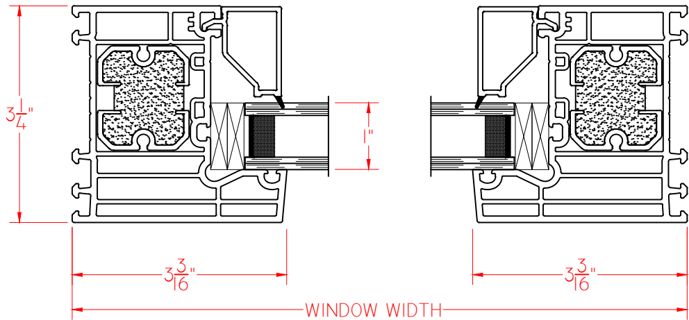
① HORIZONTAL CROSS SECTION
