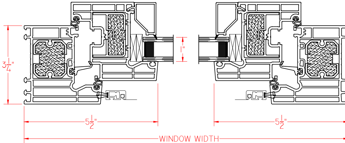
① HORIZONTAL CROSS SECTION
