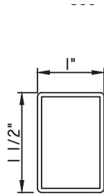
1\"X1 1/2\" TUBING MAX3016
