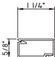
5/8"X1 1/4" SNAP TRIM MAX13827 - BASE CLIP MAX13828 - TRIM
