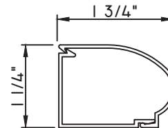
1 3/4"X1 1/4" SNAP TRIM
