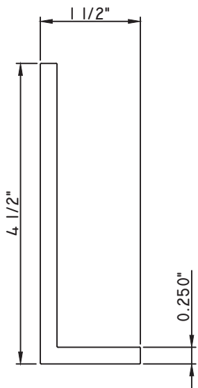
1 1/2\"X4 1/2\" ANGLE M13404
