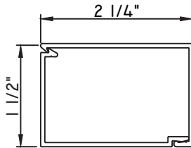
1 1/2"X2 1/4" SNAP TRIM
