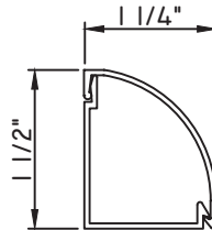
1 1/4"X1 1/2" SNAP TRIM
