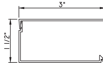
1 1/2"X3" SNAP TRIM
