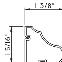
1 3/8"X1 5/16" SNAP TRIM
