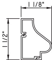
1 1/8"X1 1/2" SNAP TRIM
