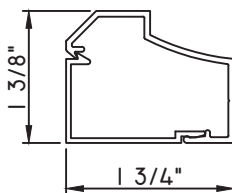
1 3/8"X1 3/4" SNAP TRIM
