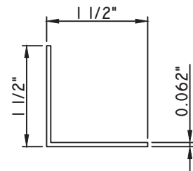
1 1/2"X1 1/2" ANGLE M13416
