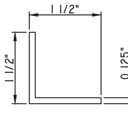
1 1/2"X1 1/2" ANGLE MW4220
