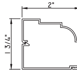
1 3/4"X2" SNAP TRIM MAX13097 - BASE CLIP M22320 - TRIM
