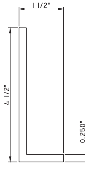
1 1/2"X4 1/2" ANGLE M13404
