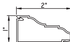
1"X2" SNAP TRIM M13097 - BASE CLIP M18975 - TRIM
