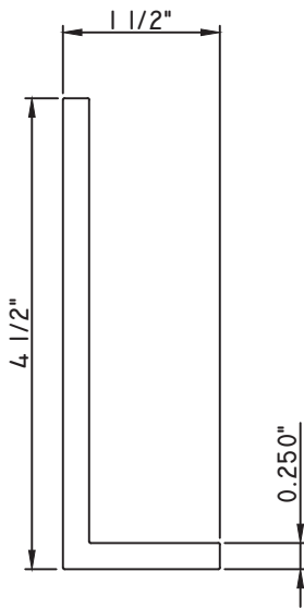
1/2"X4 1/2" ANGLE M13404
