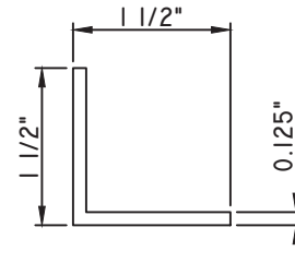
1 1/2"X1 1/2" ANGLE MW4220
