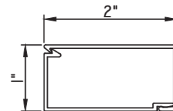
1"X2" SNAP TRIM MAX13097 - BASE CLIP MAX13098 - TRIM
