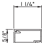
5/8"X1 1/4" SNAP TRIM MAX13827 - BASE CLIP MAX13828 - TRIM
