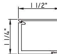
1 1/4"X1 1/2" SNAP TRIM HEAVY BASE CLIP M17072 - BASE CLIP M15267 - TRIM
