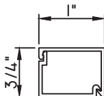
3/4"X1" SNAP TRIM M22378 - BASE CLIP M22379 - TRIM
