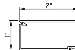
1"X2" SNAP TRIM MAX13097 - BASE CLIP MAX13098 - TRIM
