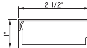
1"X2 1/2" SNAP TRIM HEAVY BASE CLIP M2272 - BASE CLIP M10120 - TRIM
