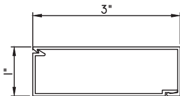
1"X3" SNAP TRIM MW24654 - BASE CLIP MW24653 - TRIM
