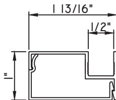
1"X1 13/16" SNAP TRIM M9762 - BASE CLIP M19848 - TRIM
