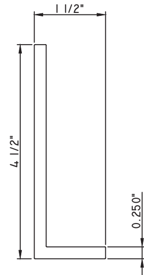
1 1/2"X4 1/2" ANGLE M13404
