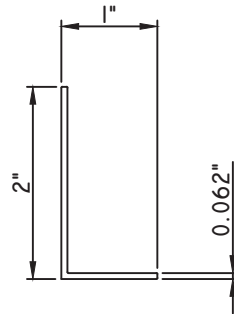
1"X2" ANGLE MW10726
