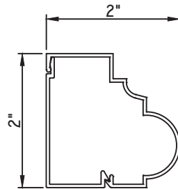
2"X2" SNAP TRIM M13097 - BASE CLIP M2215 - TRIM
