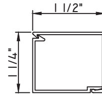
1 1/4"X1 1/2" SNAP TRIM M15266 - BASE CLIP M15267 - TRIM
