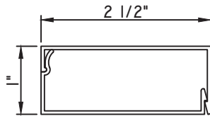
1"X2 1/2" SNAP TRIM M10121 - BASE CLIP M10120 - TRIM
