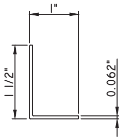
1"X1 1/2" ANGLE MAX4050
