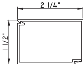
1 1/2"X2 1/4" SNAP TRIM M1984 - BASE CLIP M1983 - TRIM
