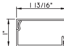
1"X1 13/16" SNAP TRIM M9762 - BASE CLIP M9761 - TRIM
