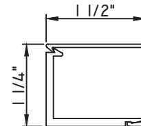
1 1/4"X1 1/2" SNAP TRIM HEAVY BASE CLIP M17072 - BASE CLIP M15267 - TRIM
