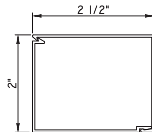
2"X2 1/2" SNAP TRIM MW23403 - BASE CLIP MW23402 - TRIM
