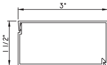
1 1/2"X3" SNAP TRIM MAX8216 - BASE CLIP MAX8215 - TRIM
