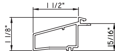
SILL NOSE D312 (WHITE) SD312 (SANDSTONE)
