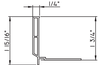
FACE FLANGE WRS-7067 (WHITE ONLY)
