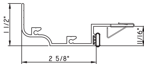
PRESET PANNING M22208 - PANNING BPN-9159 - W.S. MH8-18X1 LP - FASTENER (QTY. 8) 1974 - CLIP (6" FROM EACH CORNER & 20" O.C.)
