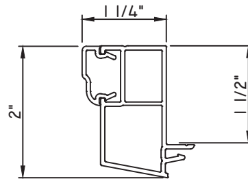
BRICKMOLD CAP: WRS-6671 (WHITE) SRS-6671 (SANDSTONE)
