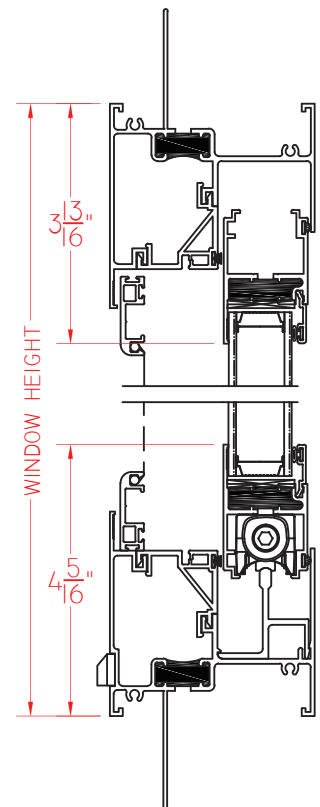
③ VERTICAL CROSS SECTION
